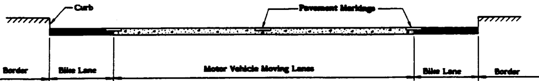
(a) Bicycle lane separated from Motor Vehicles by Pavement Markings.
