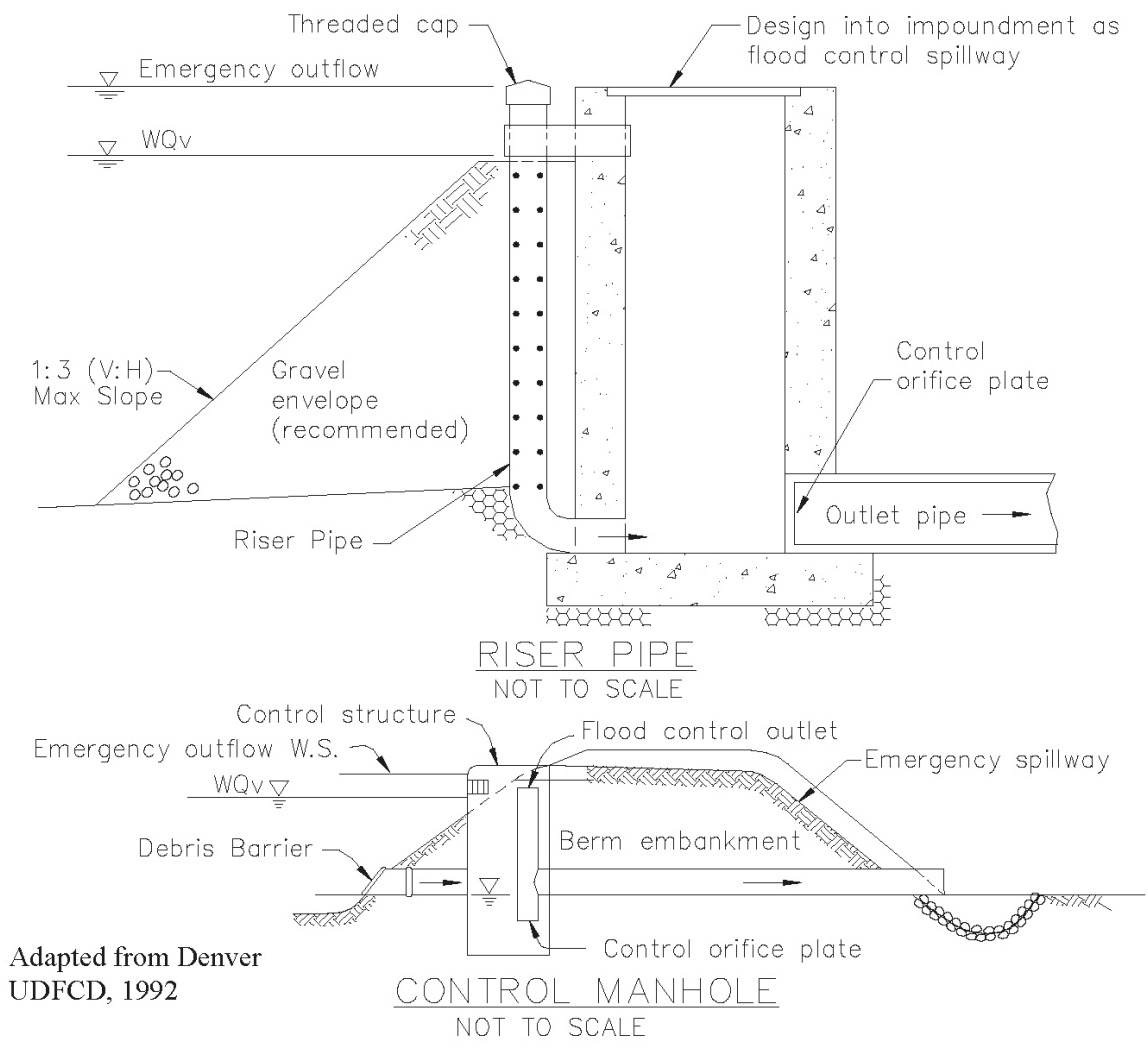
Figure 8.23 - Sandpipe Outlet Structure
