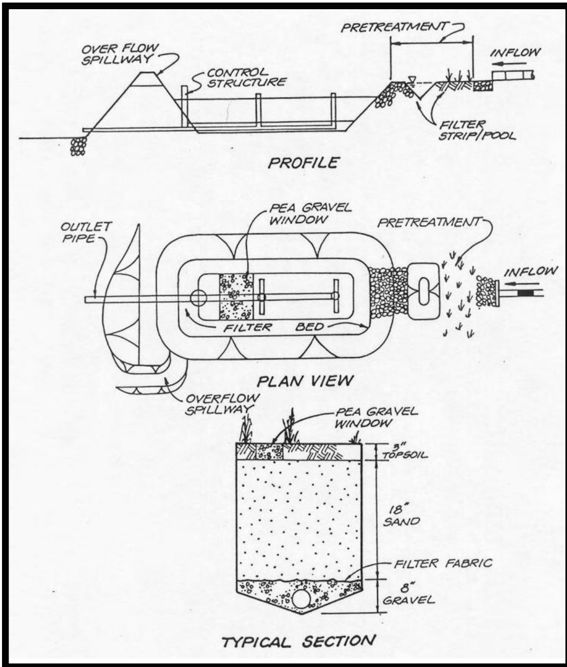
FIGURE 8.12 - Pocket Sand Filter Plan and Profile Example (for informational purposes only)
