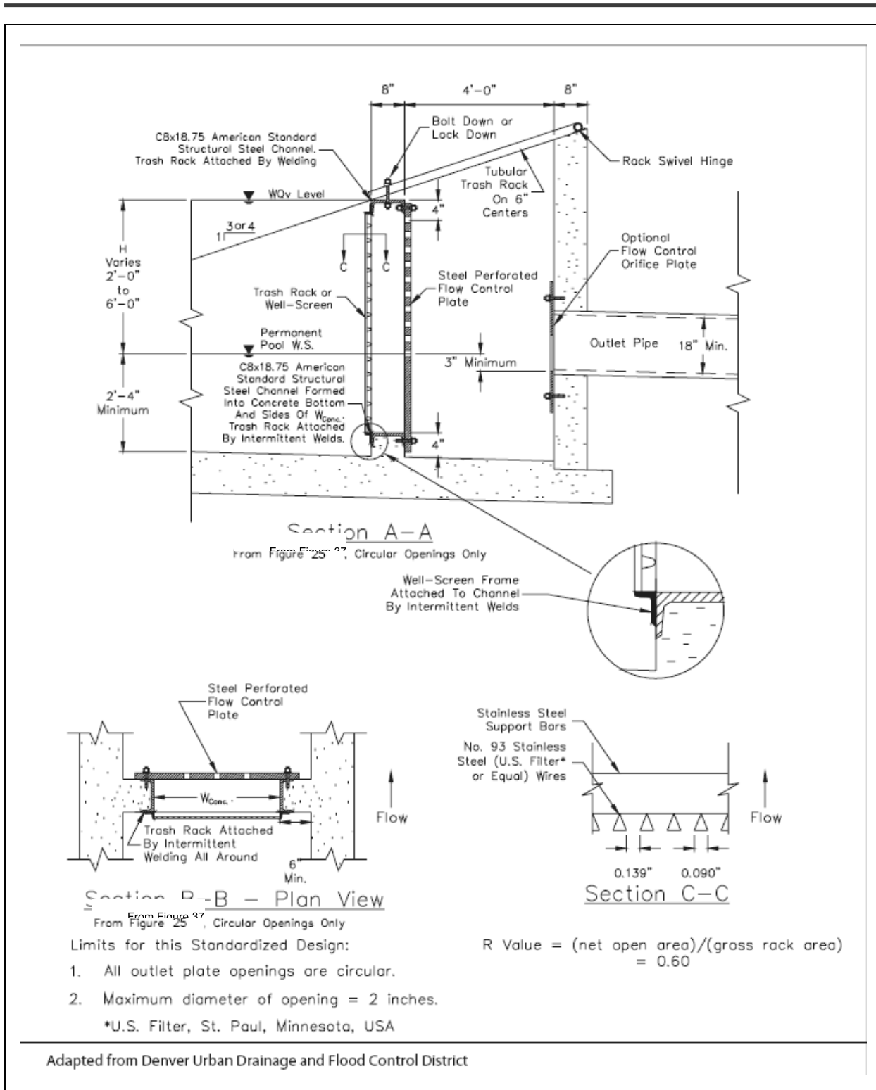
Figure 8.19 - WQv Outlet Trash Rack Design (2)
