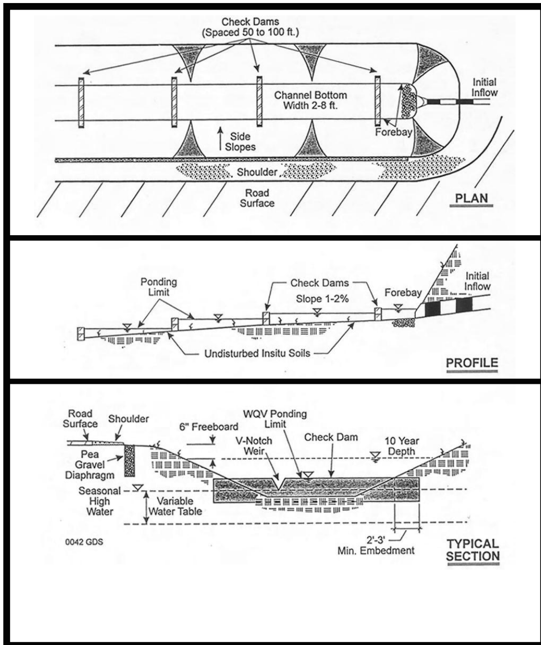
FIGURE 8.13 - Wetland Swale Plan and Profile Example (for informational purposes only)
