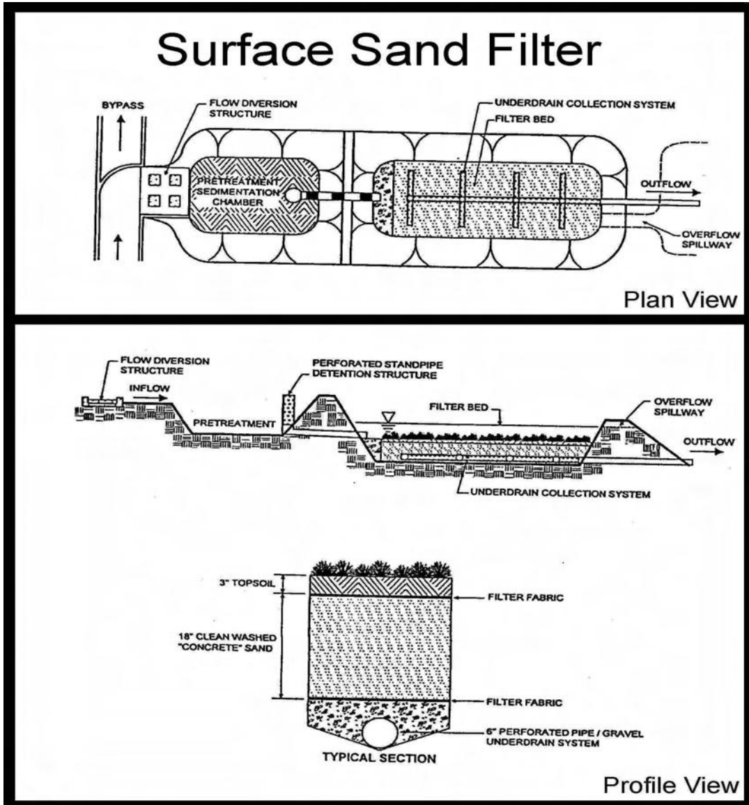
Figure 8.10 - Surface Sand Filter Plan and Profile Example (for informational purposes only)
