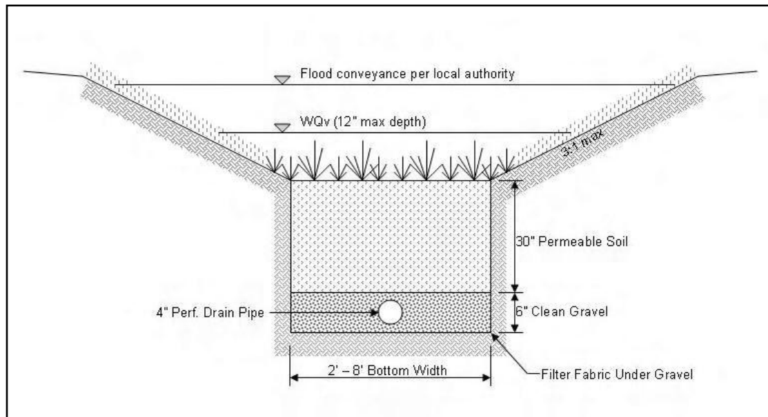
Figure 8.16 - Typical Bioswale Section
