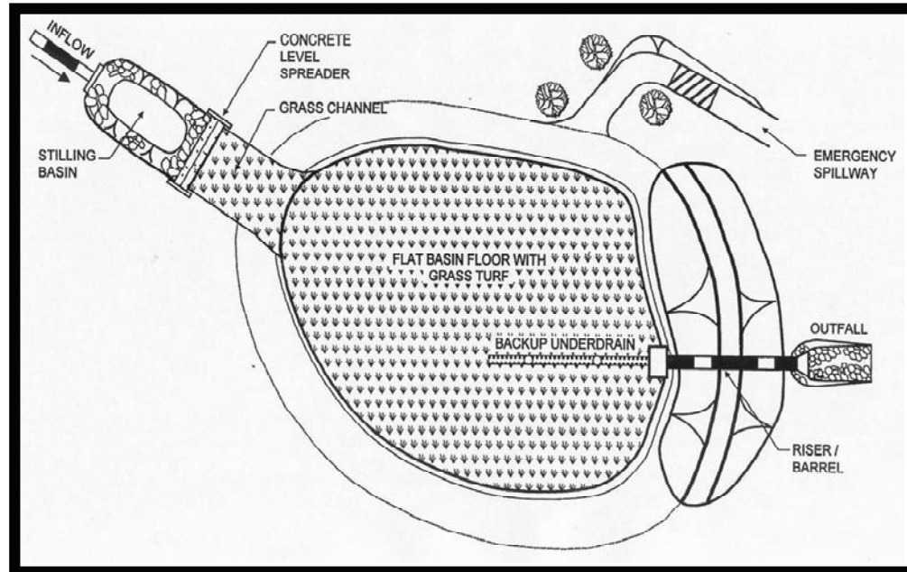
FIGURE 8.3 - Typical Infiltration Basin (for informational purposes only)
