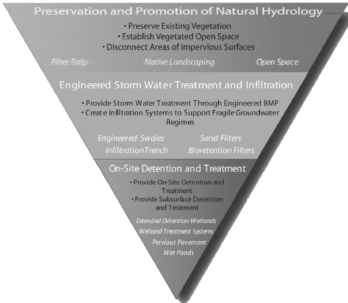
FIGURE 3.2 - Hierarchy of Stormwater Best Management Practices
