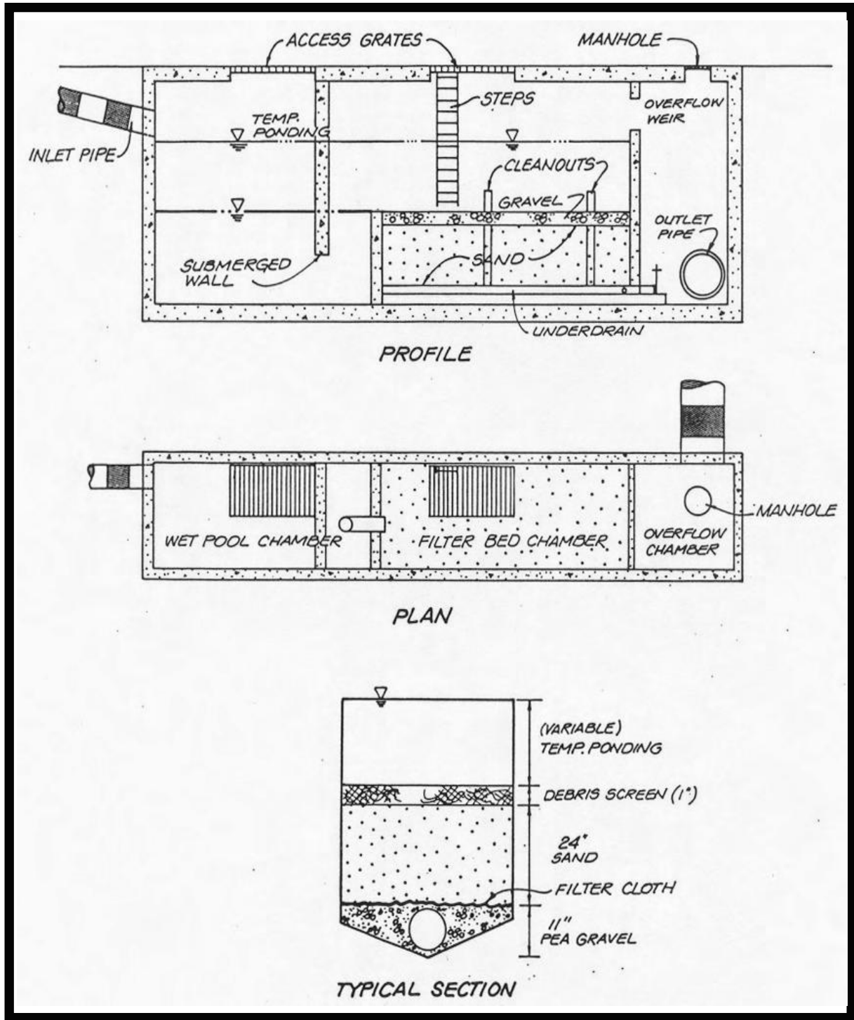
Figure 8.11 - Underground Sand Filter Plan and Profile Example (for informational purposes only)
