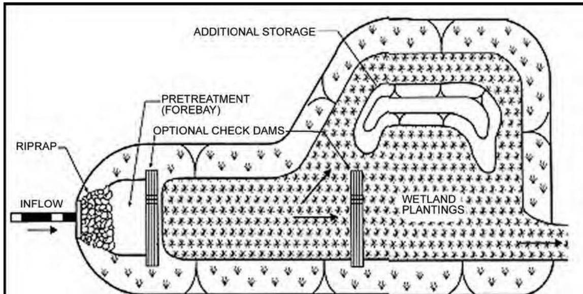
FIGURE 8.14 - Wetland Swale
