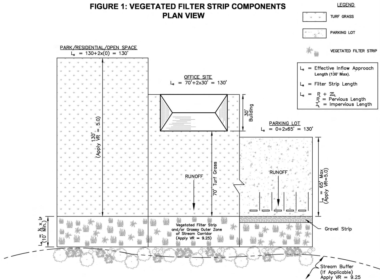
Figure 8.27 - Vegetative Filter Strip
