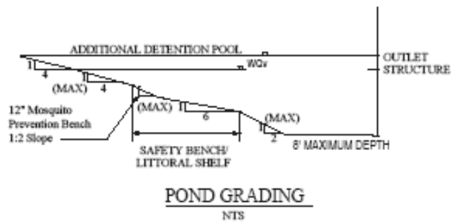
Figure 8.24 - "V" Notch Weir Outlet Structure (3)
