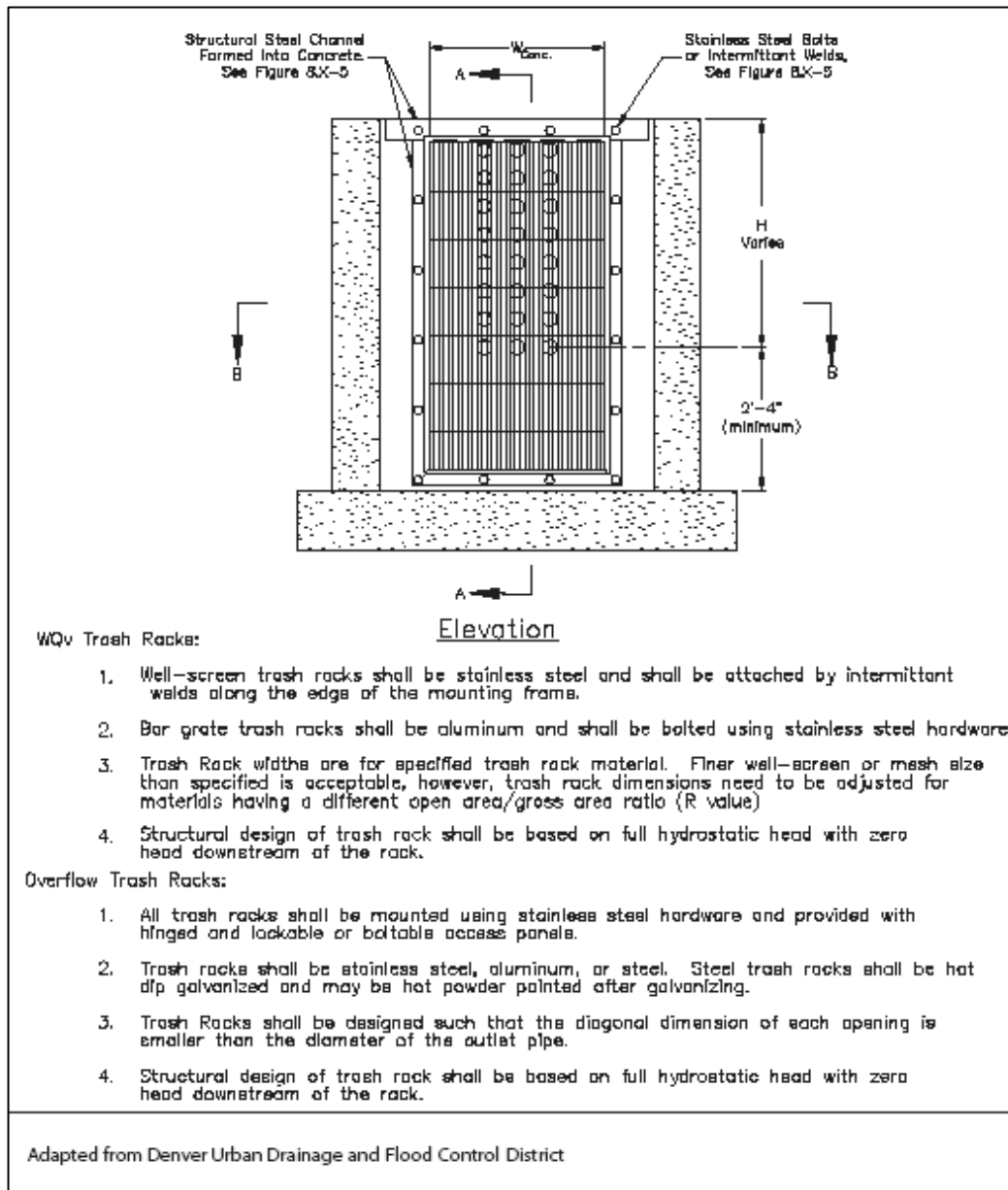
Figure 8.18 - WQv Outlet Trash Rack Design (2)
