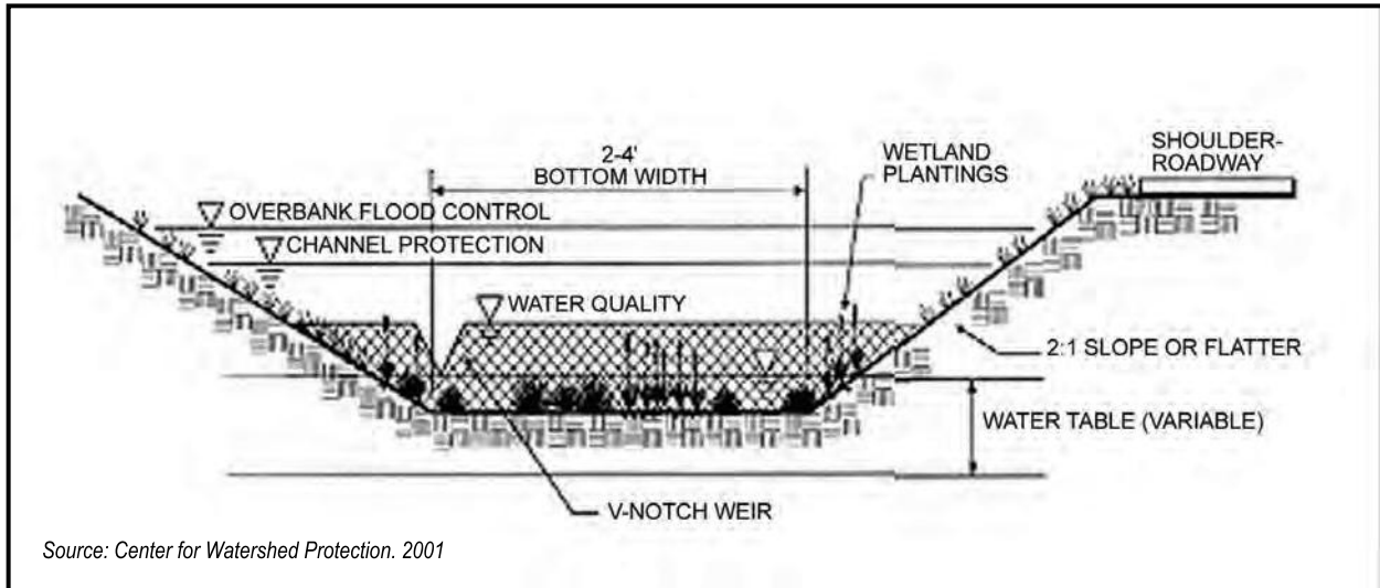
FIGURE 8.15 - Typical Wetland Swale Cross Section
